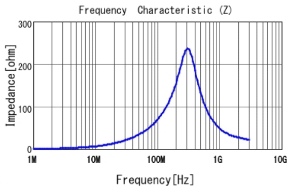
LQM2MPZR10MJH |Z|
