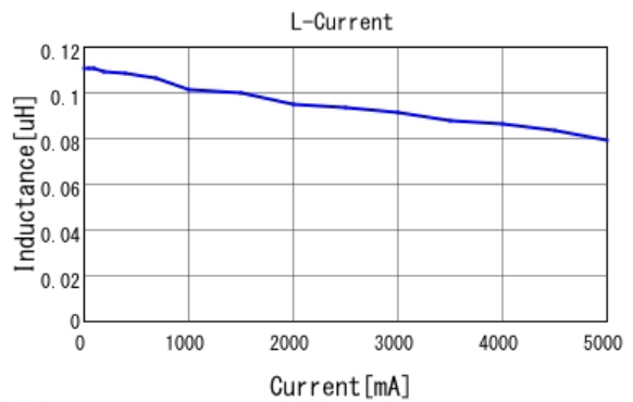
LQM2MPZR10MJH L-Current 20degC
