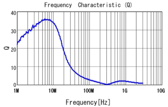
LQM2MPZR10MJH Q
