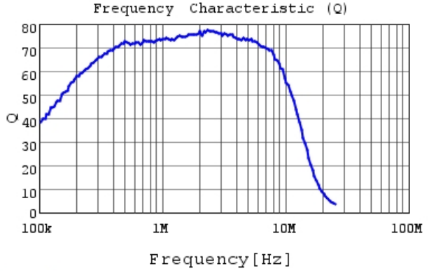
LQM2MPN4R7NG0 Q
