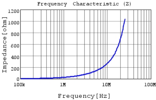
LQM2MPN4R7NG0 |Z|
