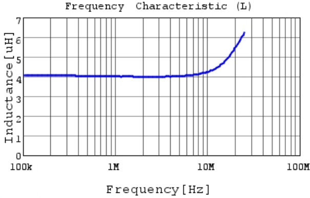
LQM2MPN4R7NG0 L
