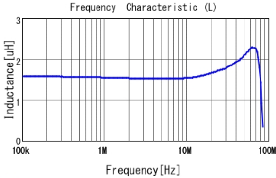
■ LQM2MPN1R5MG0 L
