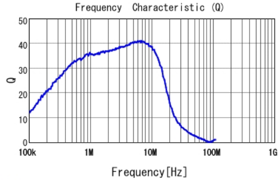
■ LQM2MPN1R5MG0 Q
