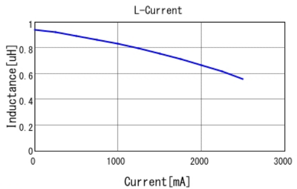
■ LQM2MPN1R0MEH L-Current 20degC
