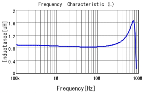
■ LQM2MPN1R0MEH L
