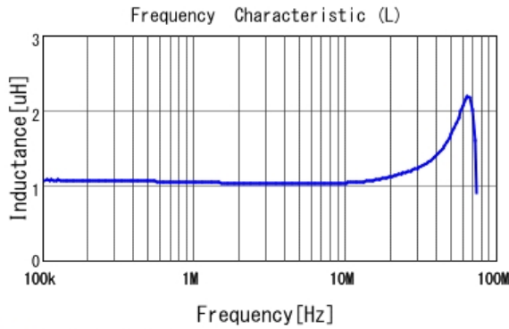
■ LQM2HPN1R0MGH L
