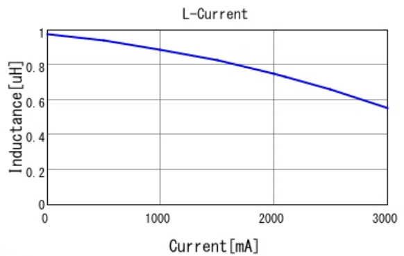
■ LQM2HPN1R0MGH L-Current 20degC
