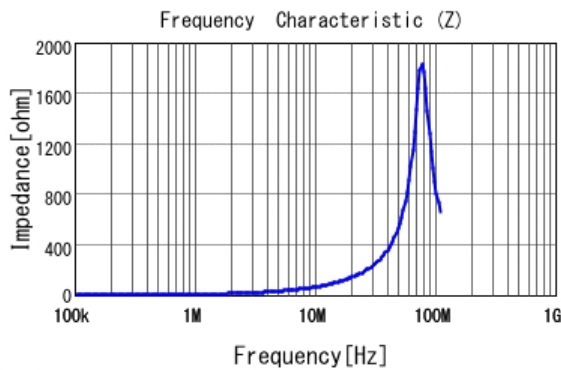
■ LQM2HPN1R0MGH |Z|
