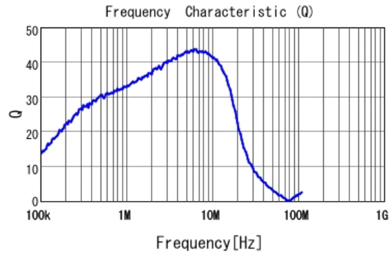
■ LQM2HPN1R0MGH Q
