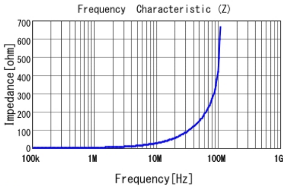
■ LQM21PNR47MGH |Z|
