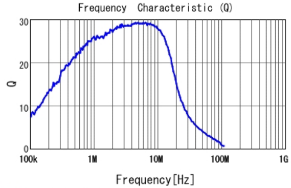
■ LQM21PNR47MGH Q
