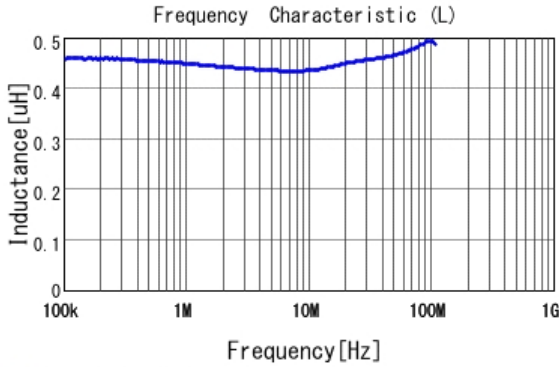
■ LQM21PNR47MGH L
