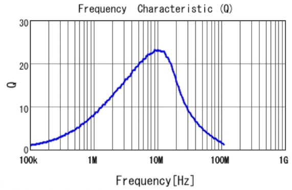
■ LQM21PNR47MEH Q
