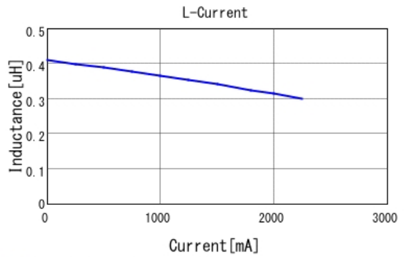
■ LQM21PNR47MEH L-Current 20degC
