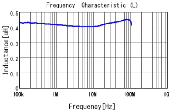
■ LQM21PNR47MEH L
