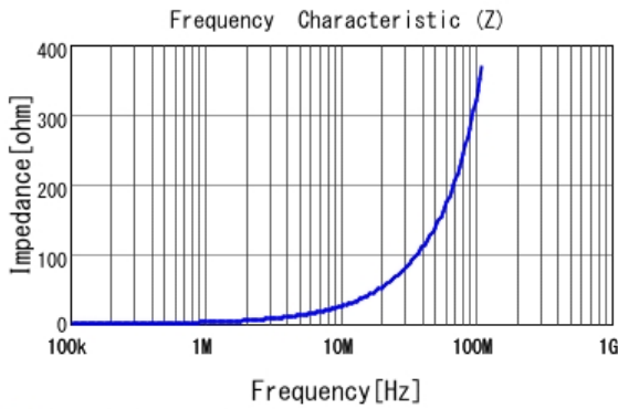
■ LQM21PNR47MEH |Z|
