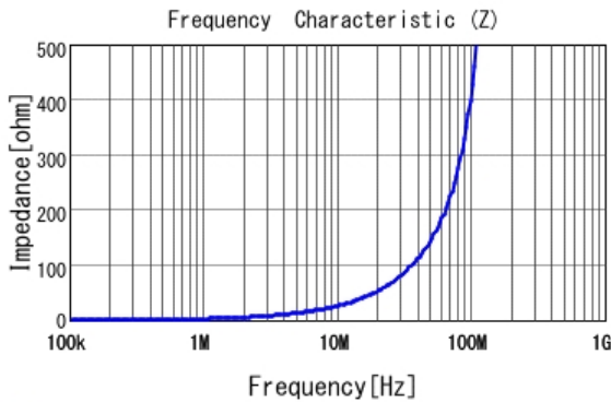
■ LQM21PNR47MCH |Z|
