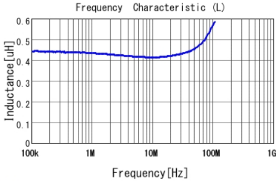
■ LQM21PNR47MCH L
