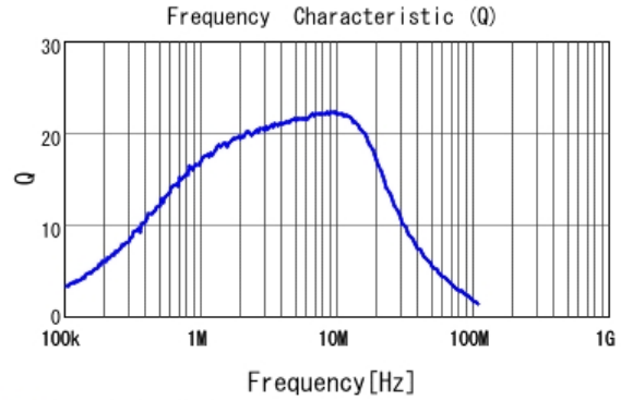
■ LQM21PNR47MCH Q
