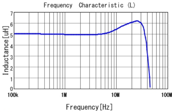
■ LQM21PN4R7MGS L
