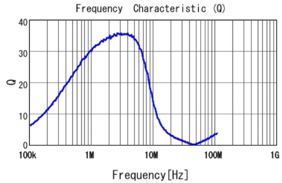
■ LQM21PN4R7MGS Q
