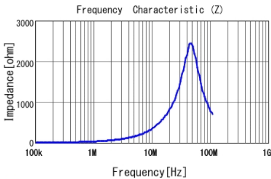
■ LQM21PN4R7MGS |Z|
