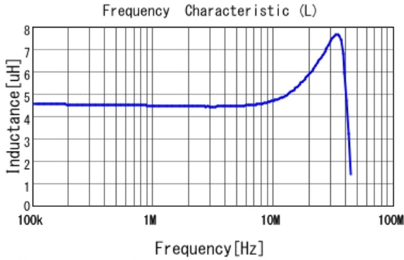
■ LQM21PN4R7MGH L
