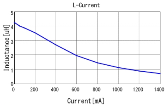
■ LQM21PN4R7MGH L-Current 20degC
