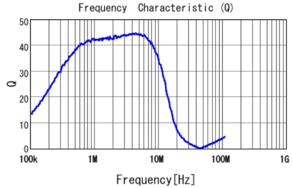
■ LQM21PN4R7MGH Q
