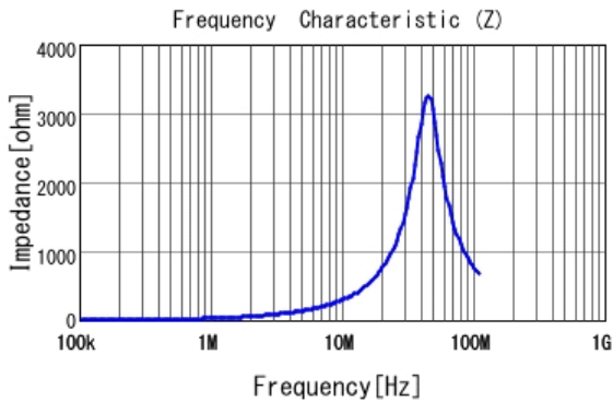
■ LQM21PN4R7MGH |Z|
