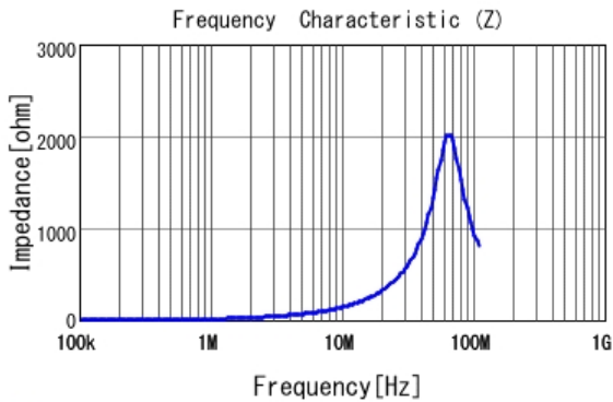
LQM21PN2R2MEH |Z|
