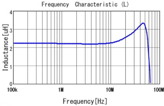
LQM21PN2R2MEH L
