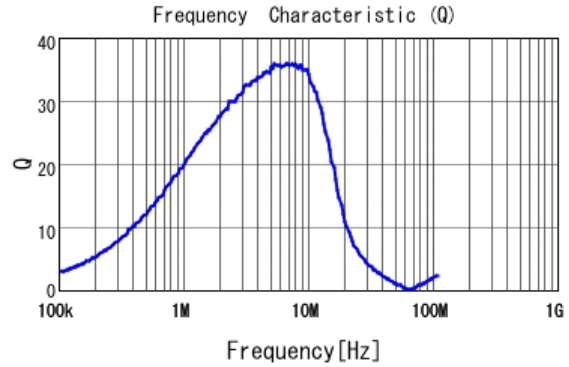
LQM21PN2R2MEH Q
