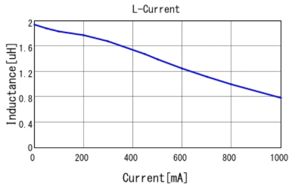
LQM21PN2R2MEH L-Current 20degC
