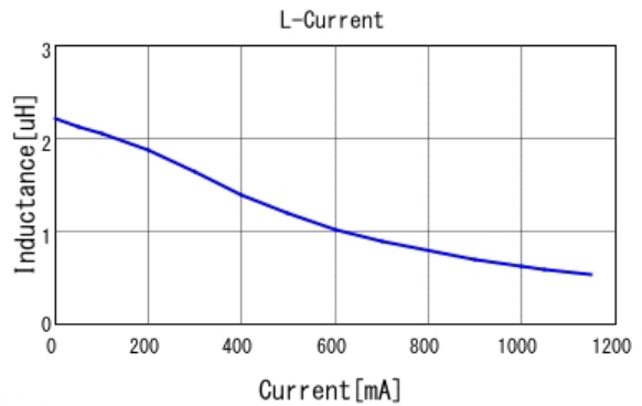
LQM21PN2R2MCA L-Current 20degC
