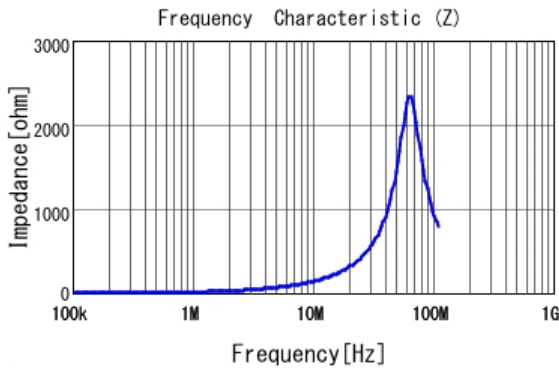
LQM21PN2R2MCA |Z|
