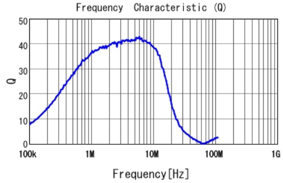
LQM21PN2R2MCA Q
