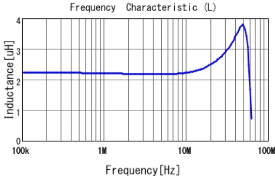
LQM21PN2R2MCA L
