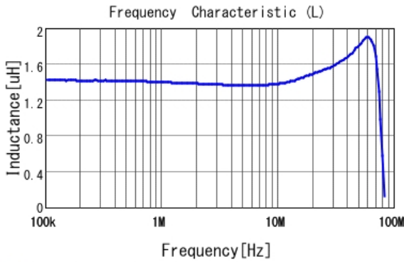
■ LQM21PN1R5MEH L
