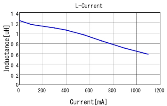
■ LQM21PN1R5MEH L-Current 20degC
