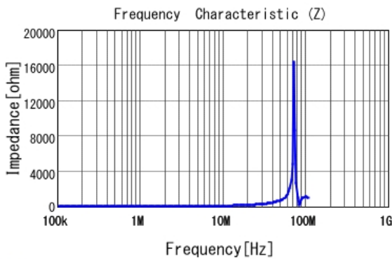
■ LQM21PN1R5MEH |Z|
