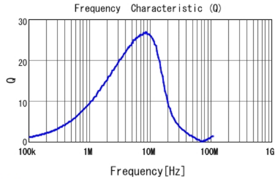
■ LQM21PN1R5MEH Q
