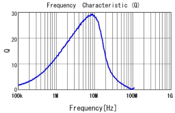
LQM21PN1R0MEH Q
