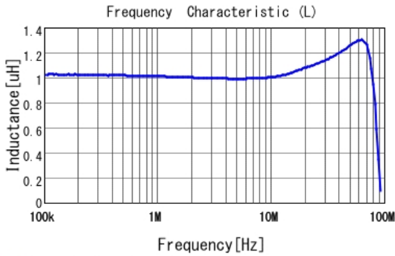
LQM21PN1R0MEH L
