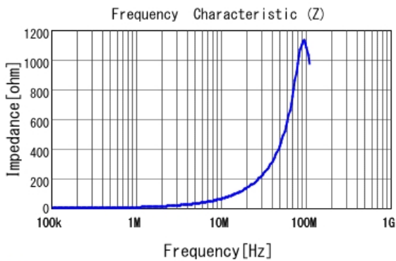
LQM21PN1R0MEH |Z|
