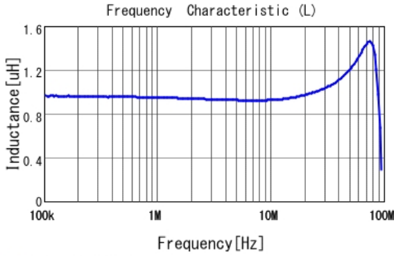
■ LQM21PN1R0MCH L
