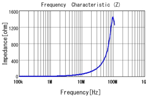
■ LQM21PN1R0MCH |Z|
