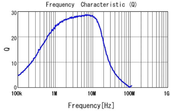
■ LQM21PN1R0MCH Q
