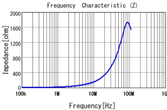
■ LQM18PZ2R2MDH |Z|
