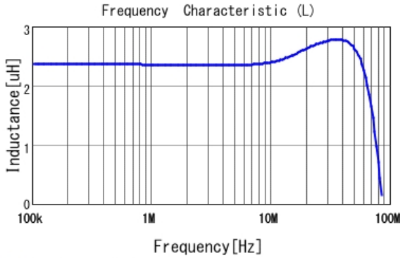
■ LQM18PZ2R2MDH L
