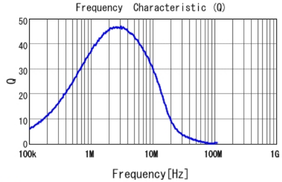
■ LQM18PZ2R2MDH Q
