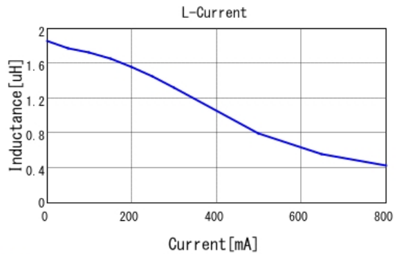
■ LQM18PZ2R2MDH L-Current 20degC
