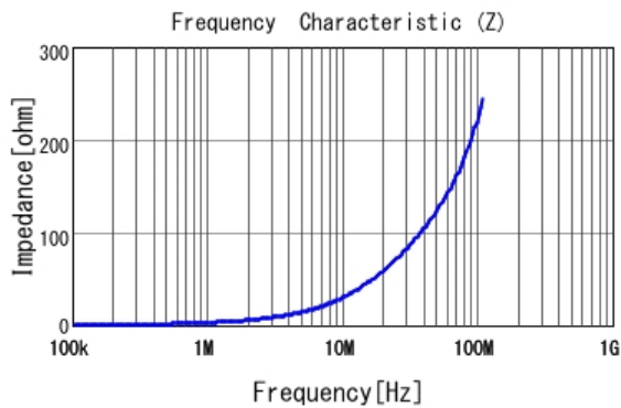
■ LQM18PNR47NC0 |Z|
