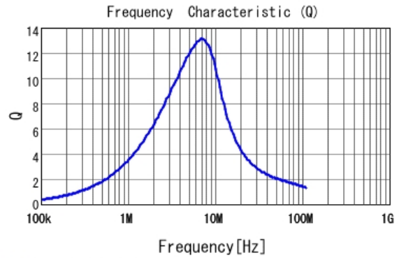
■ LQM18PNR47NC0 Q
