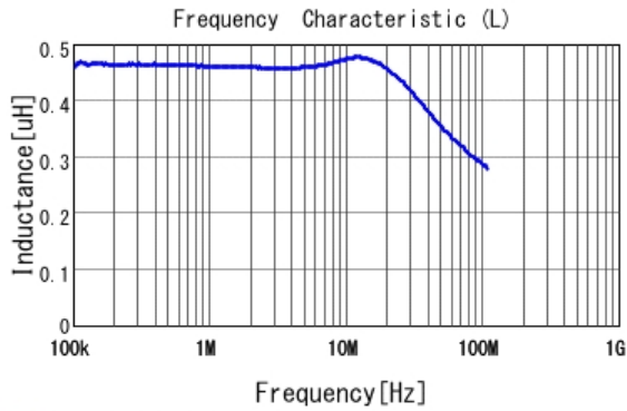
■ LQM18PNR47NC0 L
