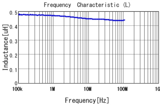
■ LQM18PNR47MFH L
