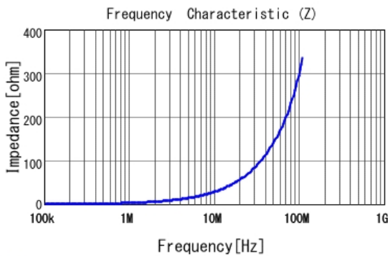
■ LQM18PNR47MFH |Z|
