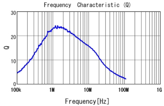
■ LQM18PNR47MFH Q
