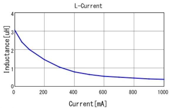
■ LQM18PN3R3MFR L-Current 20degC
