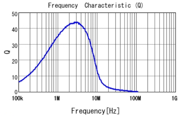
■ LQM18PN3R3MFR Q
