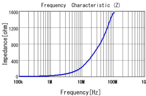
■ LQM18PN3R3MFR |Z|
