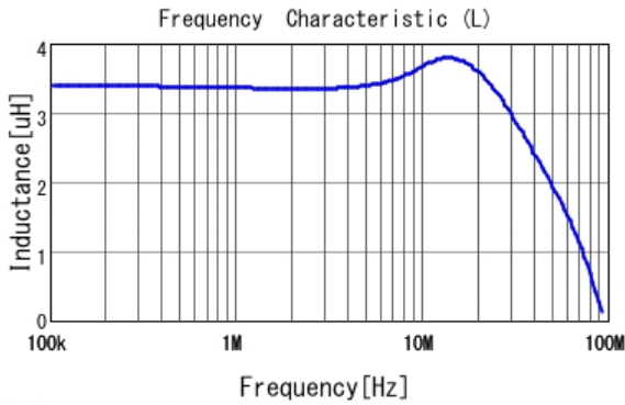
■ LQM18PN3R3MFR L
