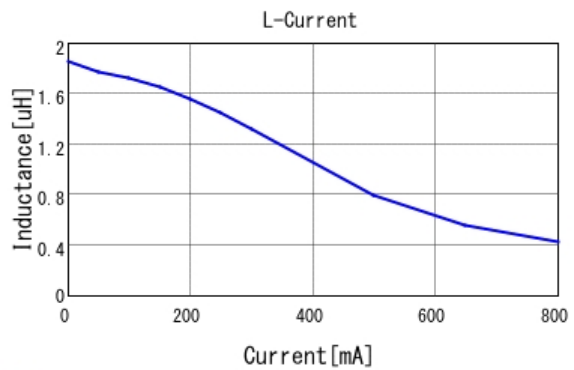
■ LQM18PN2R2MDH L-Current 20degC
