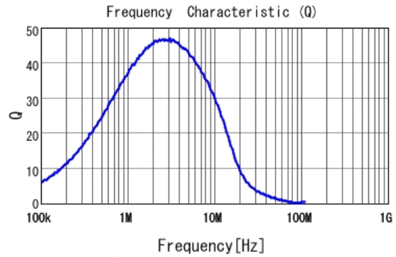
■ LQM18PN2R2MDH Q
