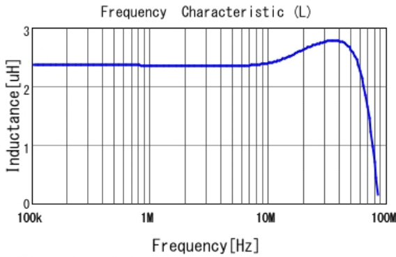
■ LQM18PN2R2MDH L
