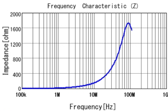
■ LQM18PN2R2MDH |Z|
