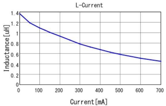
■ LQM18PN1R8NC0 L-Current 20degC
