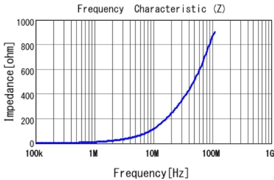
■ LQM18PN1R8NC0 |Z|
