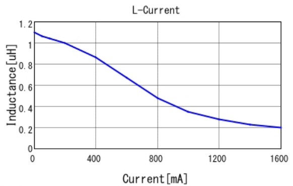
■ LQM18PN1R0MFH L-Current 20degC
