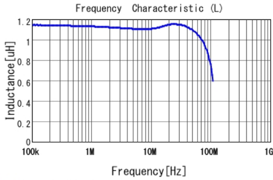
■ LQM18PN1R0MFH L
