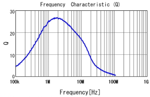
■ LQM18PN1R0MFH Q
