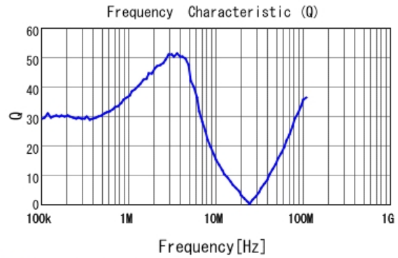
■ LQH5BPN6R8M38 Q
