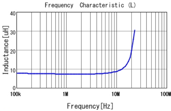
■ LQH5BPN6R8M38 L
