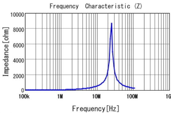
■ LQH5BPN6R8M38 |Z|
