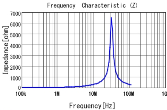
■ LQH5BPN4R7N38 |Z|
