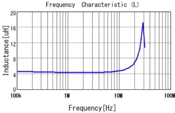
■ LQH5BPN4R7N38 L
