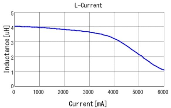
■ LQH5BPN4R7N38 L-Current 20degC
