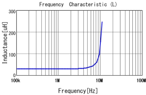
■ LQH5BPN330M38 L
