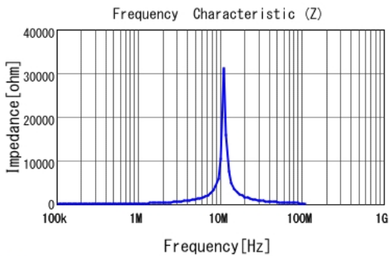
■ LQH5BPN330M38 |Z|
