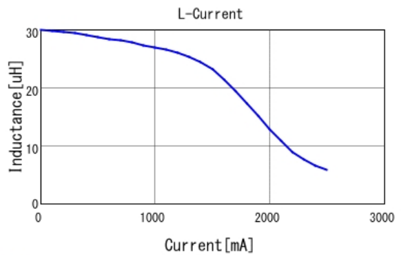
■ LQH5BPN330M38 L-Current 20degC
