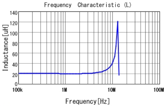
■ LQH5BPN220M38 L
