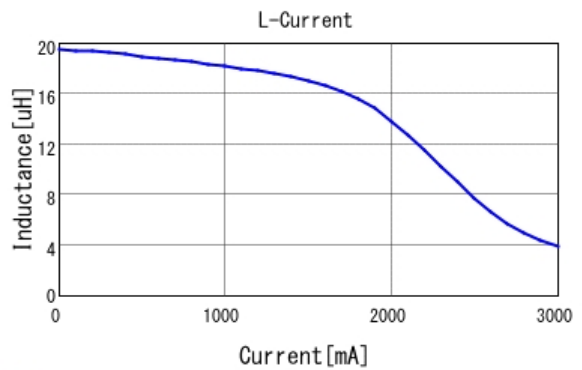
■ LQH5BPN220M38 L-Current 20degC
