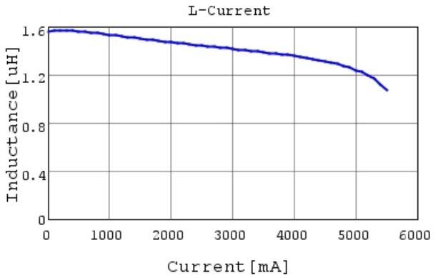
LQH5BPN1R5NT0 L-Current 20degC
