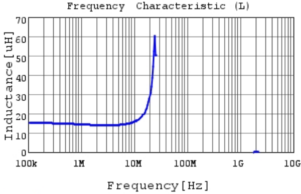
LQH5BPN150MT0 L
