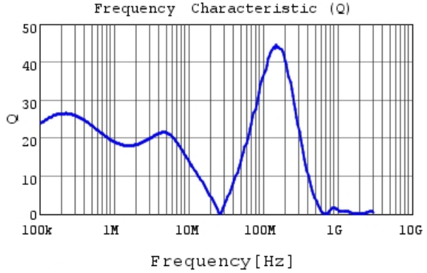
LQH5BPN150MT0 Q
