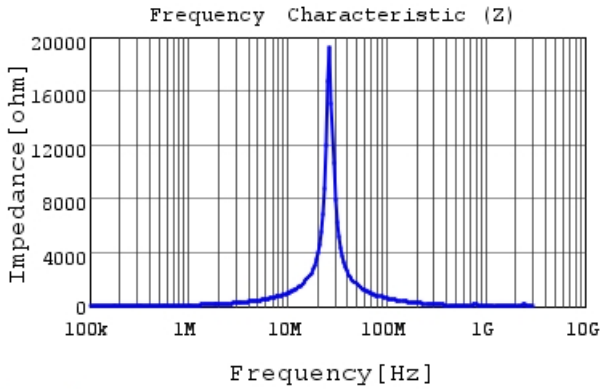
LQH5BPN150MT0 |Z|
