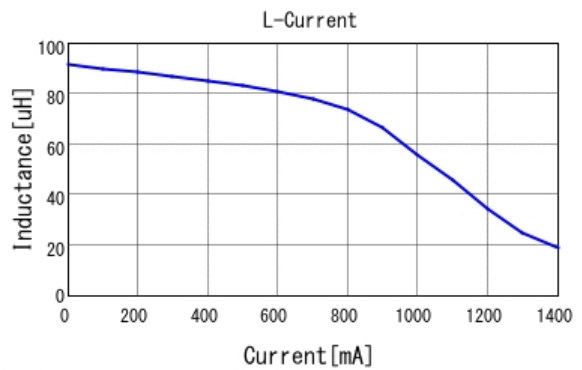
■ LQH5BPN101M38 L-Current 20degC
