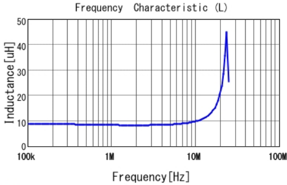
■ LQH5BPN100M38 L
