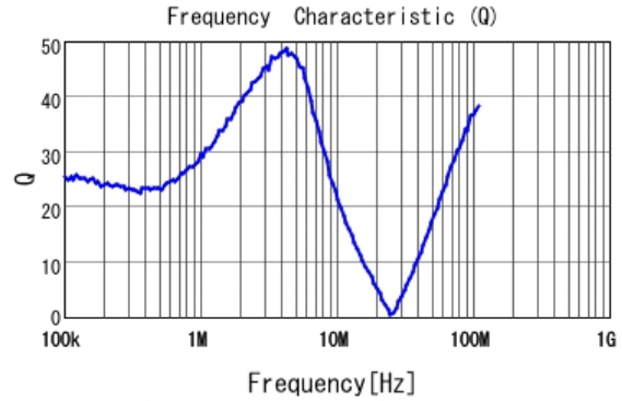
■ LQH5BPN100M38 Q
