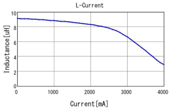
■ LQH5BPN100M38 L-Current 20degC
