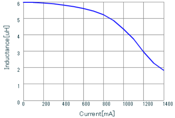
LQH44PN6R8MGR DC-Bias, 20
