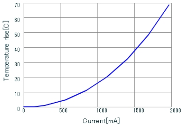
LQH44PN6R8MGR DT_Current
