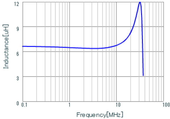
LQH44PN6R8MGR L
