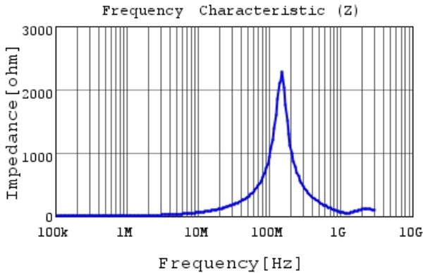
LQH43PN1R0N26 |Z|
