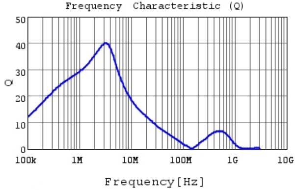
LQH43PN1R0N26 Q
