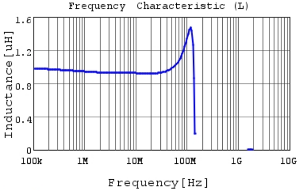
LQH43PN1R0N26 L
