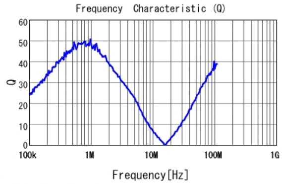
■ LQH3NPZ470MME Q
