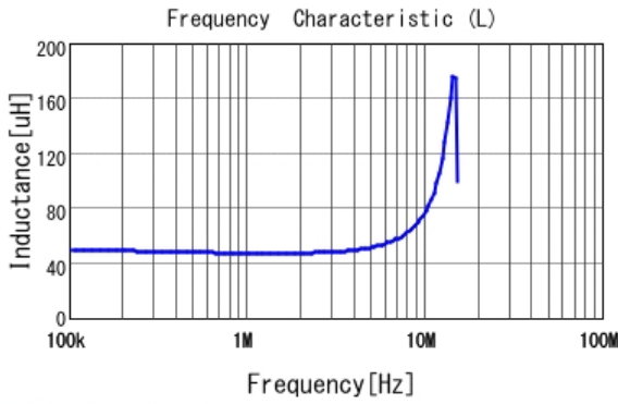
■ LQH3NPZ470MME L
