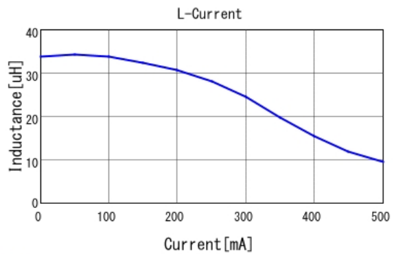
■ LQH3NPZ330MGR L-Current 20degC
