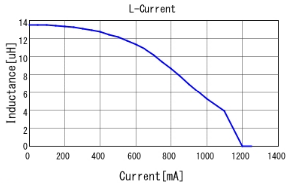
■ LQH3NPZ150MME L-Current 20degC
