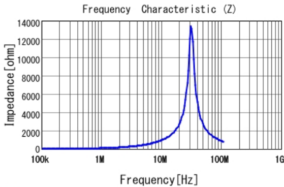
■ LQH3NPZ150MME |Z|
