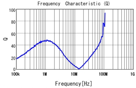
■ LQH32PZ101MN0 Q
