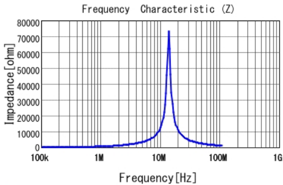
■ LQH32PZ101MN0 |Z|
