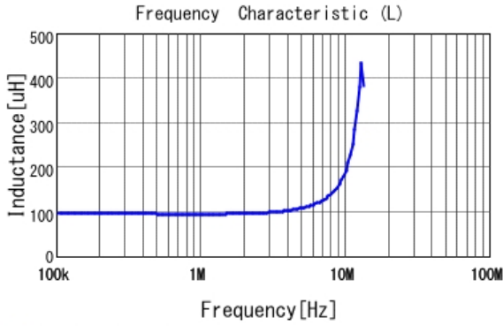
■ LQH32PZ101MN0 L
