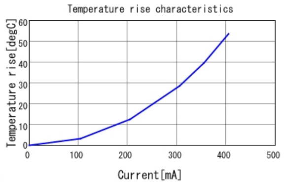
■ LQH32PN470MN0 Temp. rise
