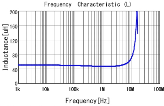
■ LQH32PN470MN0 L
