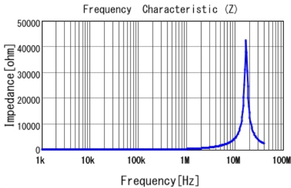
■ LQH32PN470MN0 |Z|
