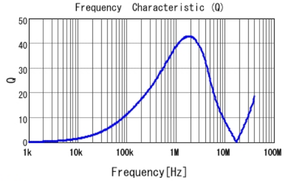
■ LQH32PN470MN0 Q
