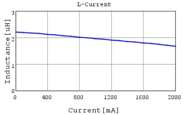
LQH32PN2R2NNC L-Current 20degC
