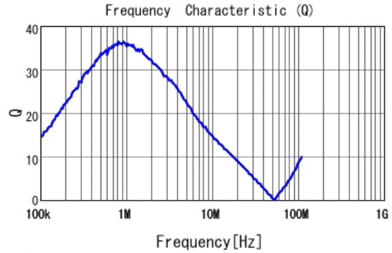
LQH32PH6R8NN0 Q
