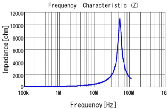
LQH32PH6R8NN0 |Z|
