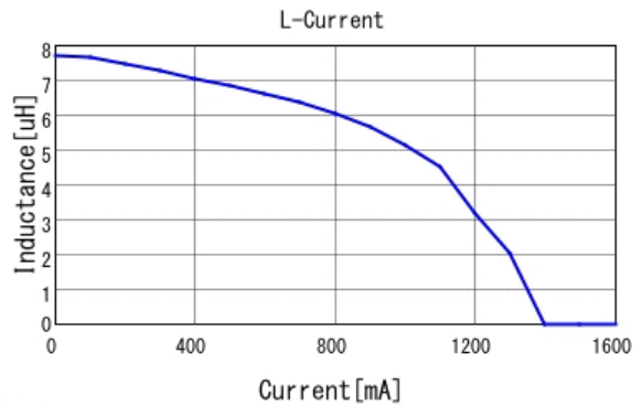
LQH32PH6R8NN0 L-Current 20degC
