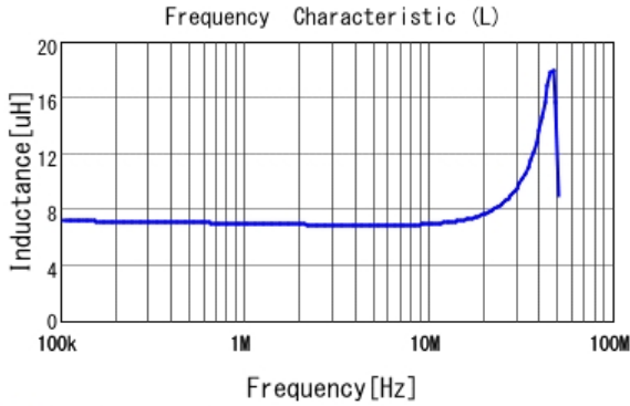
LQH32PH6R8NN0 L
