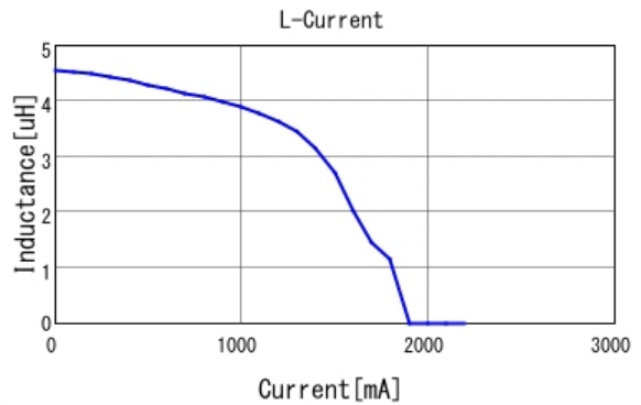
LQH32PB4R7NN0 L-Current 20degC
