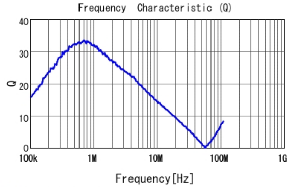
LQH32PB4R7NN0 Q
