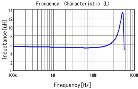
LQH32PB4R7NN0 L
