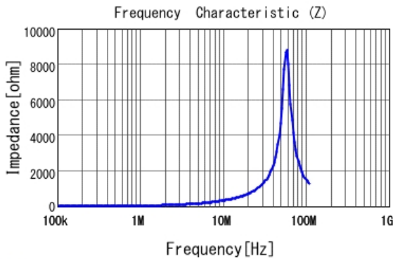
LQH32PB4R7NN0 |Z|
