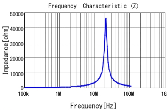
■ LQH32PB470MN0 |Z|
