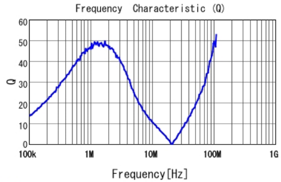
■ LQH32PB470MN0 Q
