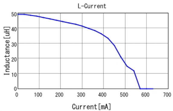
■ LQH32PB470MN0 L-Current 20degC
