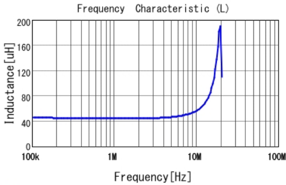
■ LQH32PB470MN0 L
