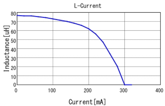
■ LQH2MPN820MGR L-Current 20degC
