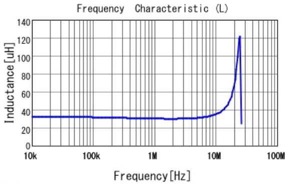
■ LQH2MPN330MGR L
