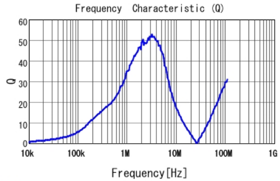
■ LQH2MPN330MGR Q
