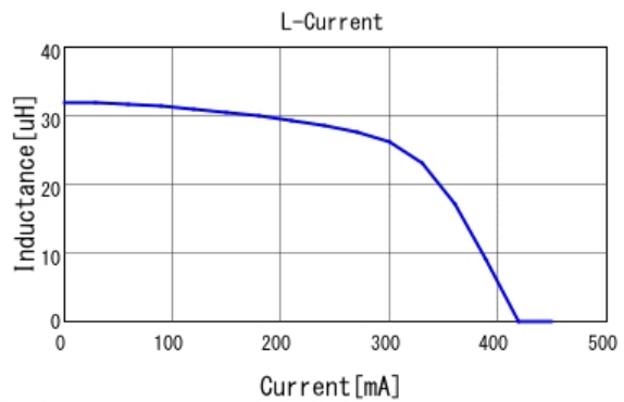
■ LQH2MPN330MGR L-Current 20degC
