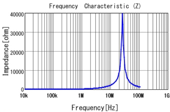
■ LQH2MPN330MGR |Z|
