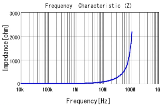
■ LQH2HPZ1R2NJR |Z|
