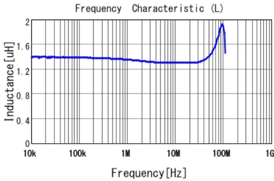
■ LQH2HPZ1R2NJR L
