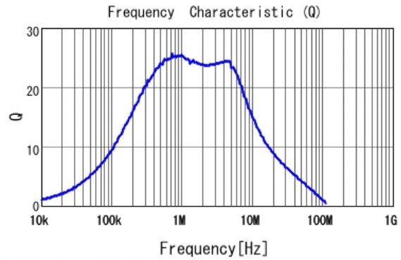
■ LQH2HPZ1R2NJR Q
