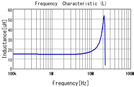
■ LQH2HPZ150MGR L
