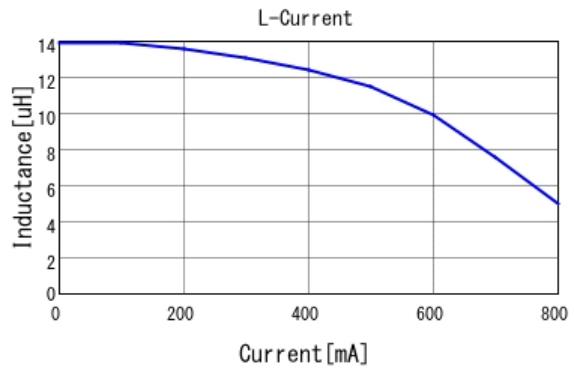
■ LQH2HPZ150MGR L-Current 20degC
