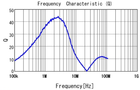
■ LQH2HPZ150MGR Q
