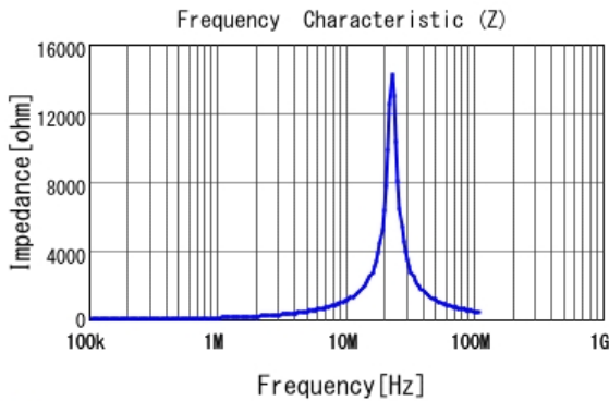
■ LQH2HPZ150MGR |Z|
