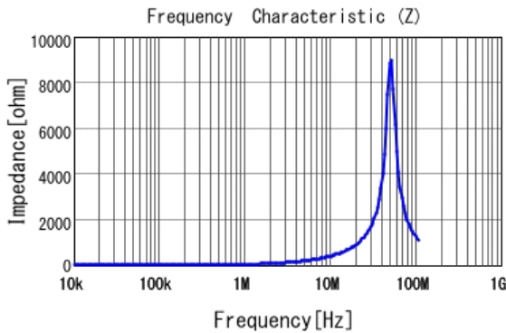
■ LQH2HPN6R8MJR |Z|
