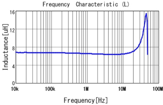
■ LQH2HPN6R8MJR L
