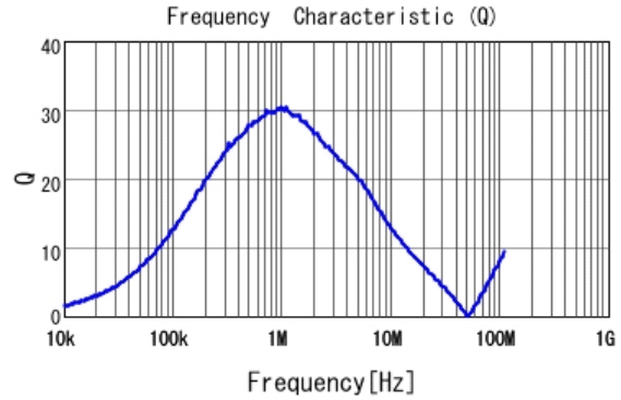
■ LQH2HPN6R8MJR Q
