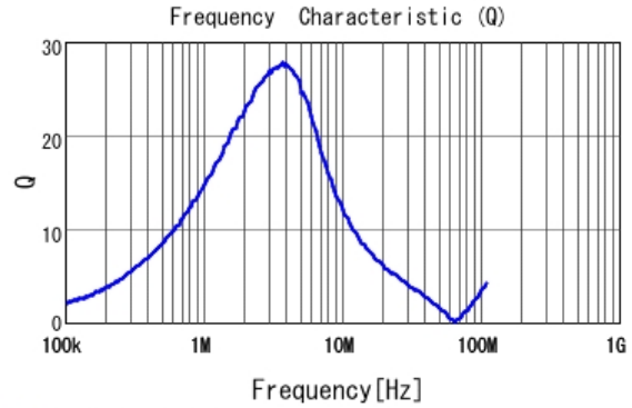
■ LQH2HPN6R8MDR Q
