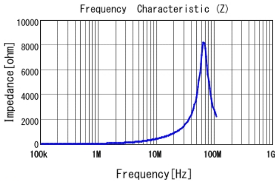
■ LQH2HPN6R8MDR |Z|
