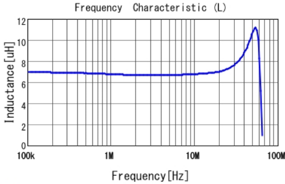
■ LQH2HPN6R8MDR L
