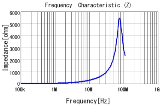
LQH2HPN4R7MDR |Z|
