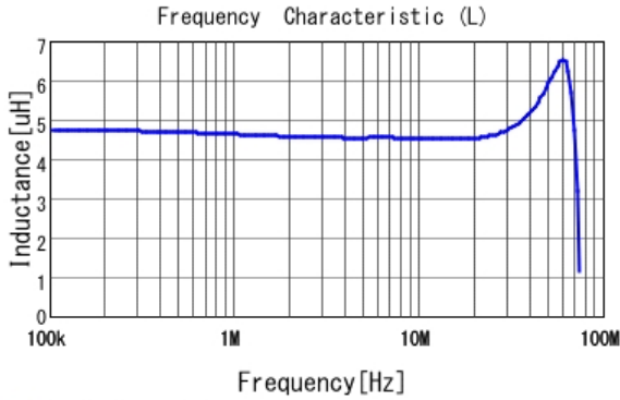
LQH2HPN4R7MDR L
