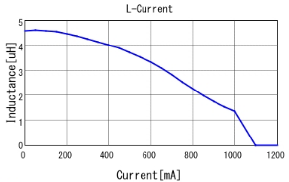
LQH2HPN4R7MDR L-Current 20degC
