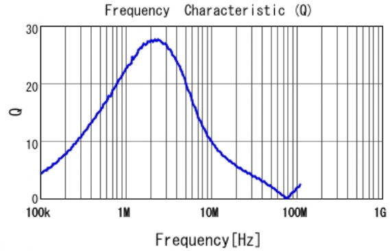
LQH2HPN4R7MDR Q
