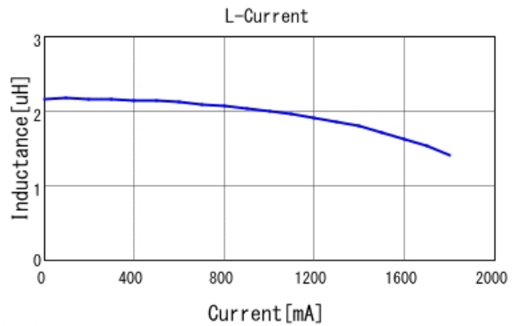
■ LQH2HPN2R2MJR L-Current 20degC
