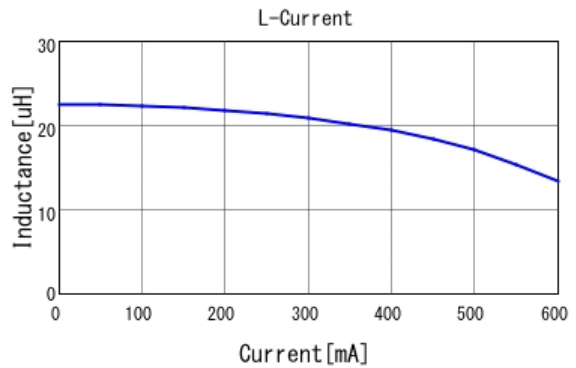
LQH2HPN220MJR L-Current 20degC
